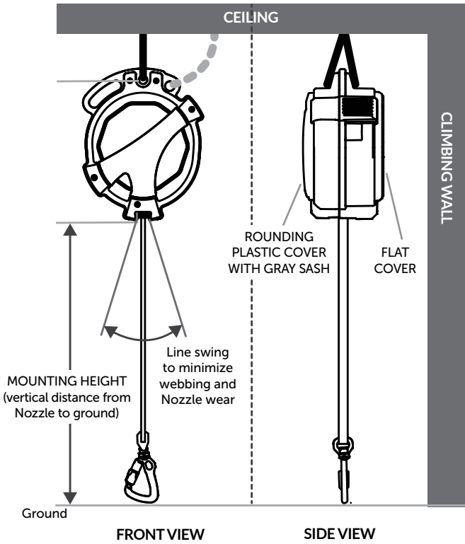
Mounting Dimensions
